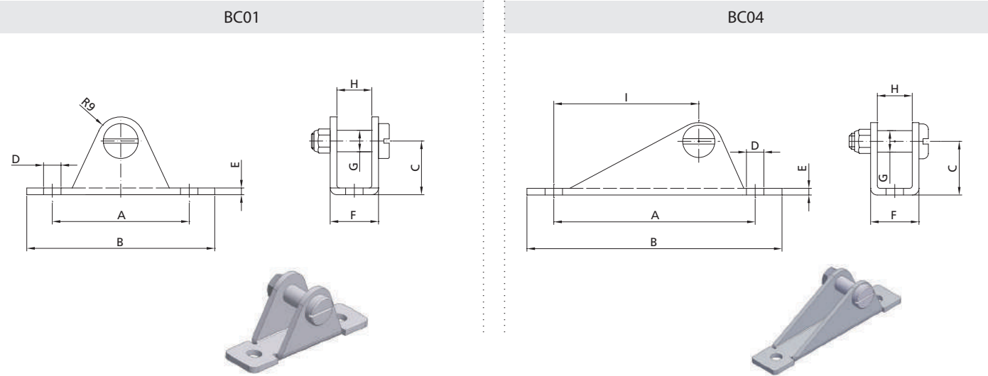
Bearing shoe
